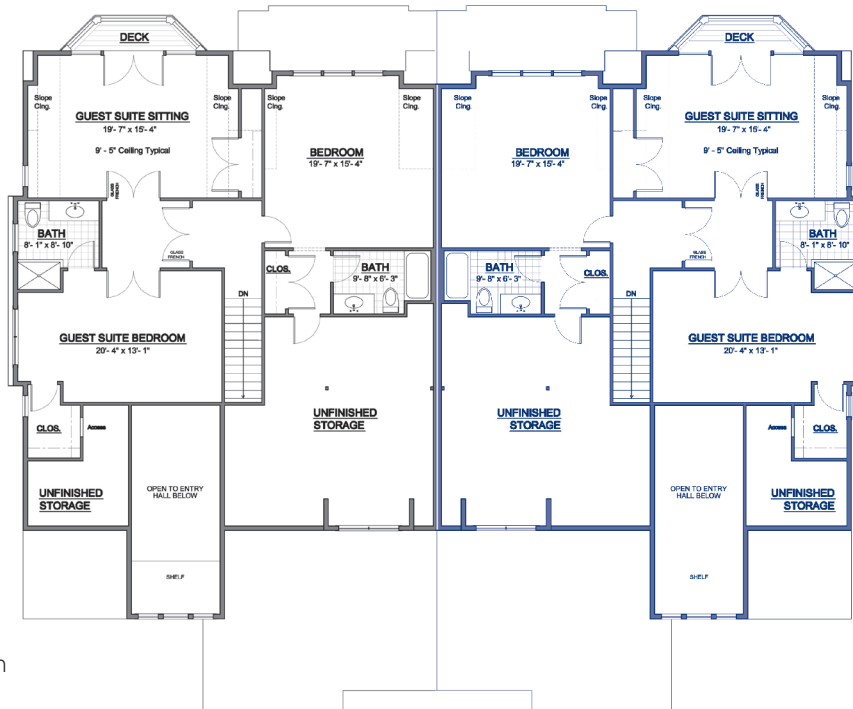
Second Floor Right Plan 1,271 S.F.
