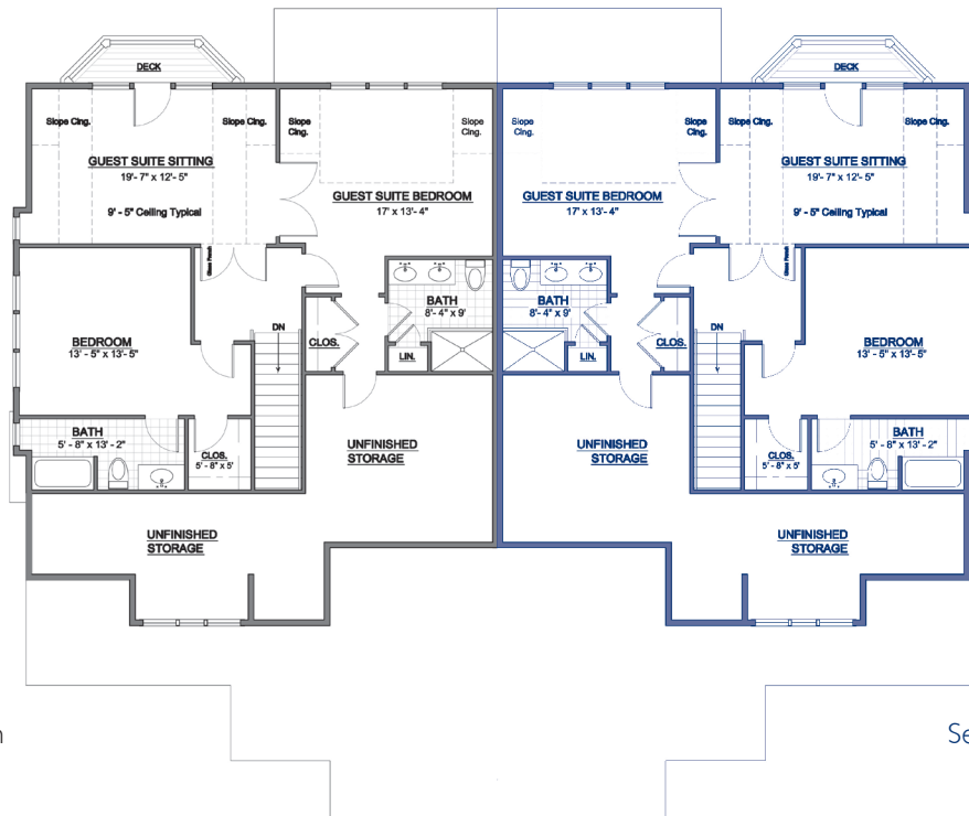
Second Floor Left Plan 1,076 S.F.
